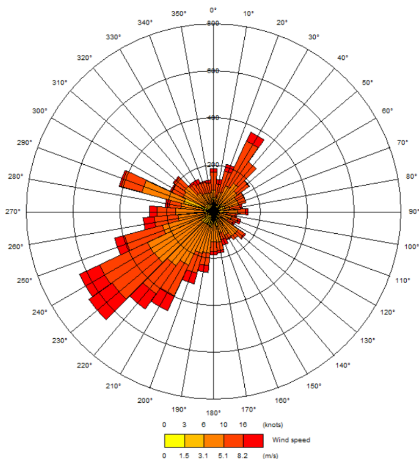
Plate 3.1 Wind Rose from Manston Airport (2023)
